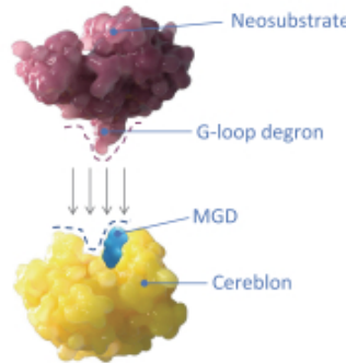
MGD-mediated cereblon-neosubstrate interaction
